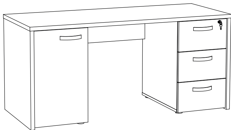
BU16 160 x 74 x 65 cm BU16+OG 160 x 136 x 67 cm
